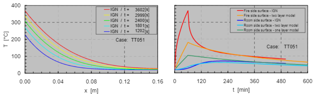
Figure 6. Results from heat transfer calculations. Left-hand side: evolution of temperature distribution inside an one-layer wall. As the firing period ends after one hour, the temperature distribution is notably non-uniform, indicating that the lumped-capacity model is inappropriate. Right-hand side: evolution of surface temperatures of the wall. For the analysis of heat transfer from the stove to the room, it is important to be able to predict the temperature of the room side surface accurately; at least for this case, surprisingly good results are obtained with the two-layer model where each of the layers is analyzed using the lumped-capacity assumption.
