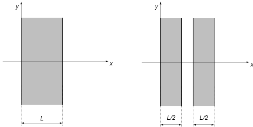
Figure 5. Two examples of simplified stove wall geometry for heat transfer calculations. Heat from the fire is transferred to the left-hand surface at x = 0 and propagates through the wall to the right-hand surface, from where it is transferred to the room by convection and radiation.
