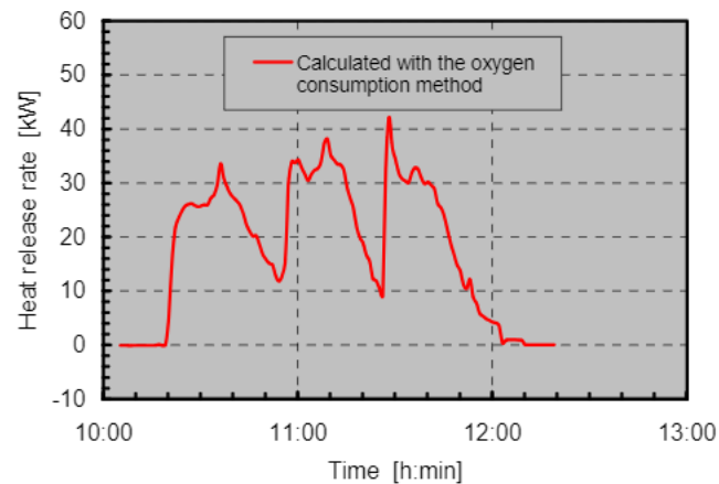
Figure 4. Heat release rate from burning firewood during a stove experiment. The heat release rate was computed from experimental data by using the oxygen consumption method. Three batches of firewood were burned in this particular experiment, and the combustion behavior of each batch exhibits the three different phases of fire development (growth phase, fully developed phase, decay phase). Details of the experiment and the calculation method are given by Paloposki et al. (in press).
