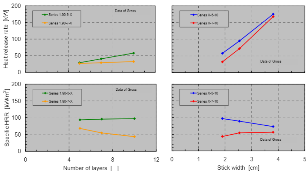
Figure 3. The maximum values of heat release rate and specific heat release rate in the experiments of Gross (1962). For the loosely packed cribs (series 1.90-5-X and X-5-10), higher values of heat release rate and specific heat release rate are observed than for the densely packed cribs (series 1.90-7-X and X-7-10). The sticks appear to shield each other from thermal radiation and to obstruct the flow of air to the surface of the sticks, thus retarding the combustion. The magnitude of the effect depends on the configuration of the crib, but seems to follow the intuition that the effect should be stronger for densely packed cribs.
